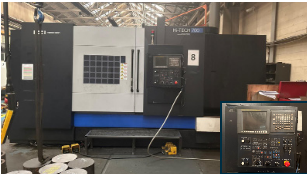
Lot 11: HWACHEON Hi-Tec 700 CNC Lathe with Fanuc Series 0i-TD Control (2014)
