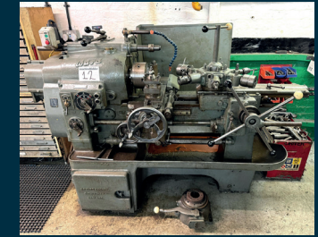
LOT 12. WARD 3C Capstan Lathe with 3 Jaw Chuck and Collet Chuck
