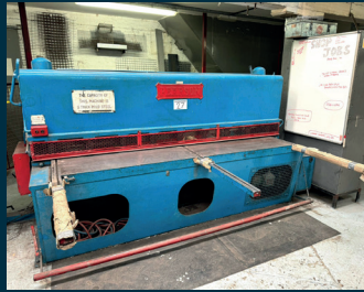
LOT 27. PEARSON 8' x 1/4" Hydraulic Guillotine
