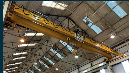
TECHNICAL CRANES 10 Ton SWL Double Girder Overhead Crane with 5 Ton Aux Hoist (main bay)
